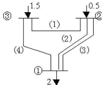
Fig1. Three lines diagram of electric power system
