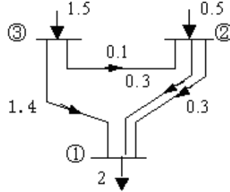
Fig2. tide of three lines of electric power system
