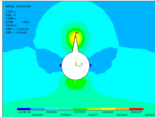
Figure 3. Comparison chart of magnetic flux density
