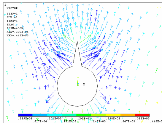
Figure 4. Comparison chart of magnetic flux density
