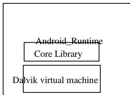
Figure 1 Android_Runtime
